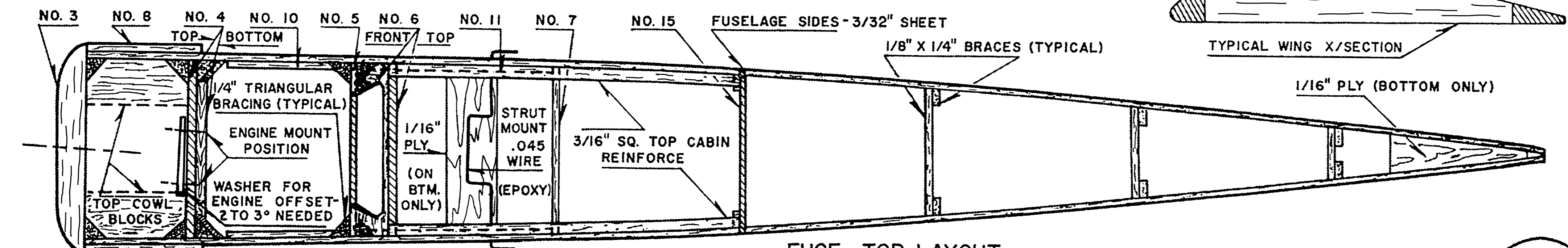
FUSE. TOP LAYOUT NOTE: TOP & BOTTOM COVERING NOT SHOWN FOR CLARITY
