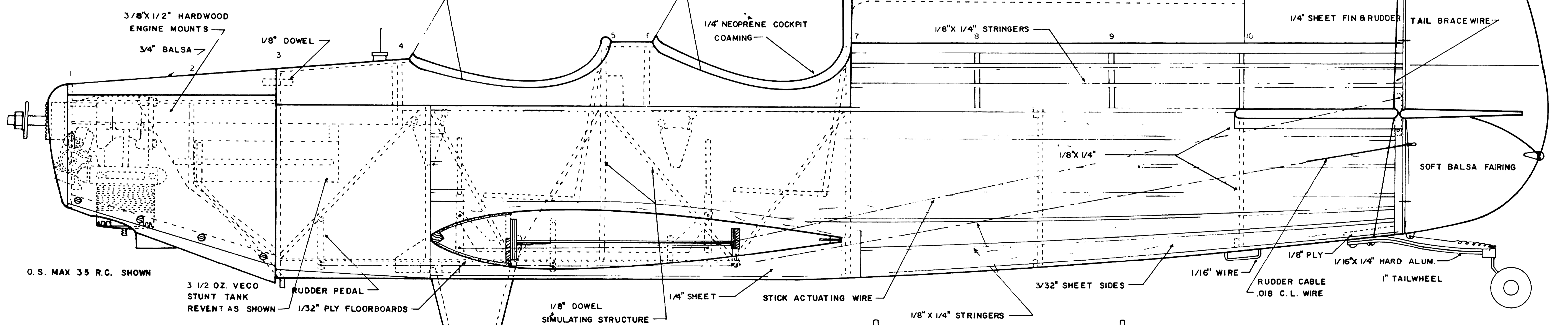
BUILD UP FROM 1/4" SHEET
