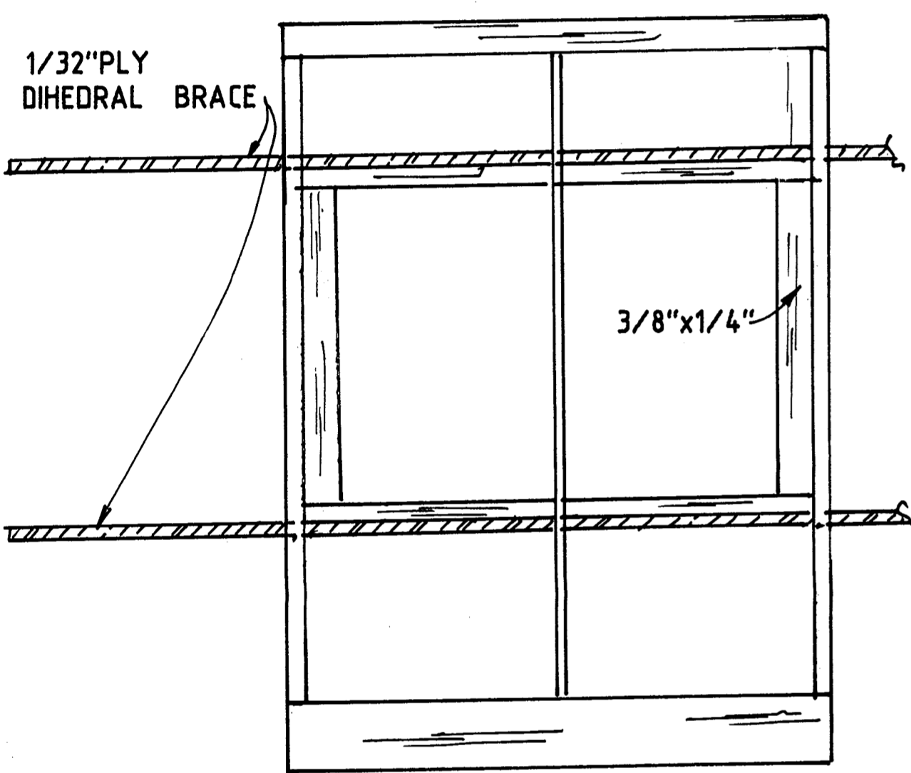
TOP WING CENTRE SECTION
