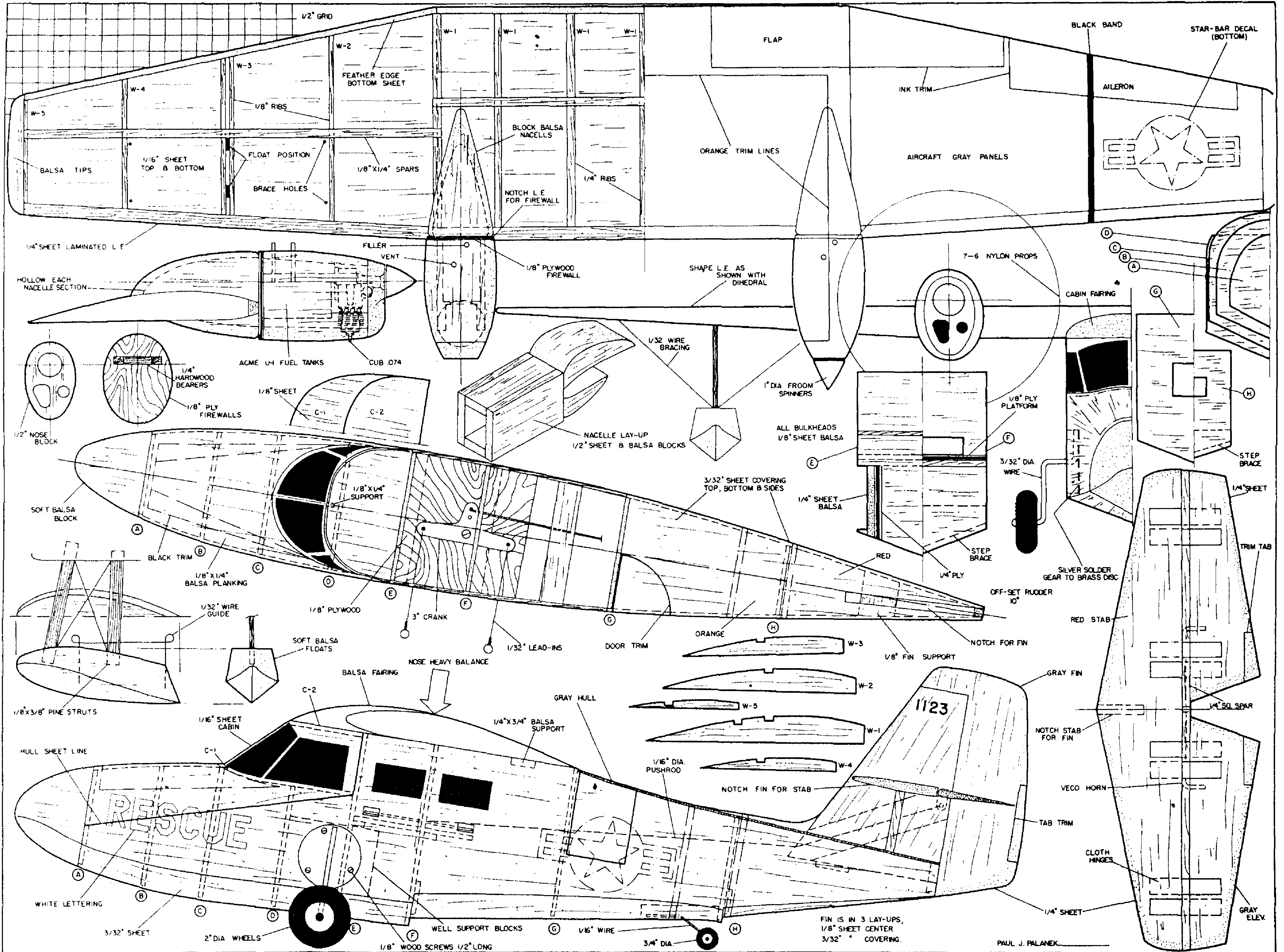
"WIDGEON" Beautiful scale amphibian for two .074's. Can use up to .15's. Controline,
