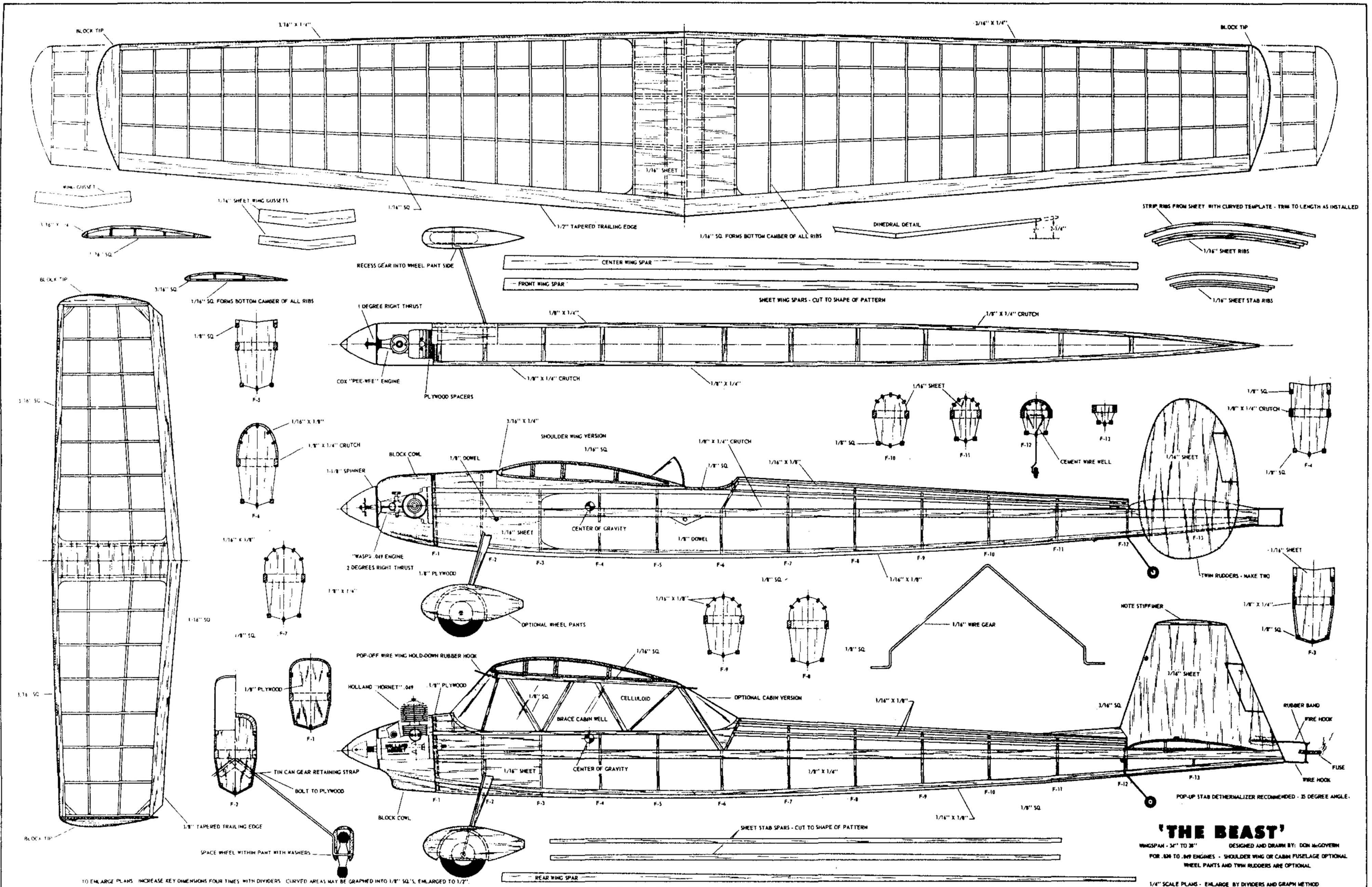
"BEAST" Shoulder wing or cabin sport free-flight, .020 to .049 engines - by Don McGovern.
