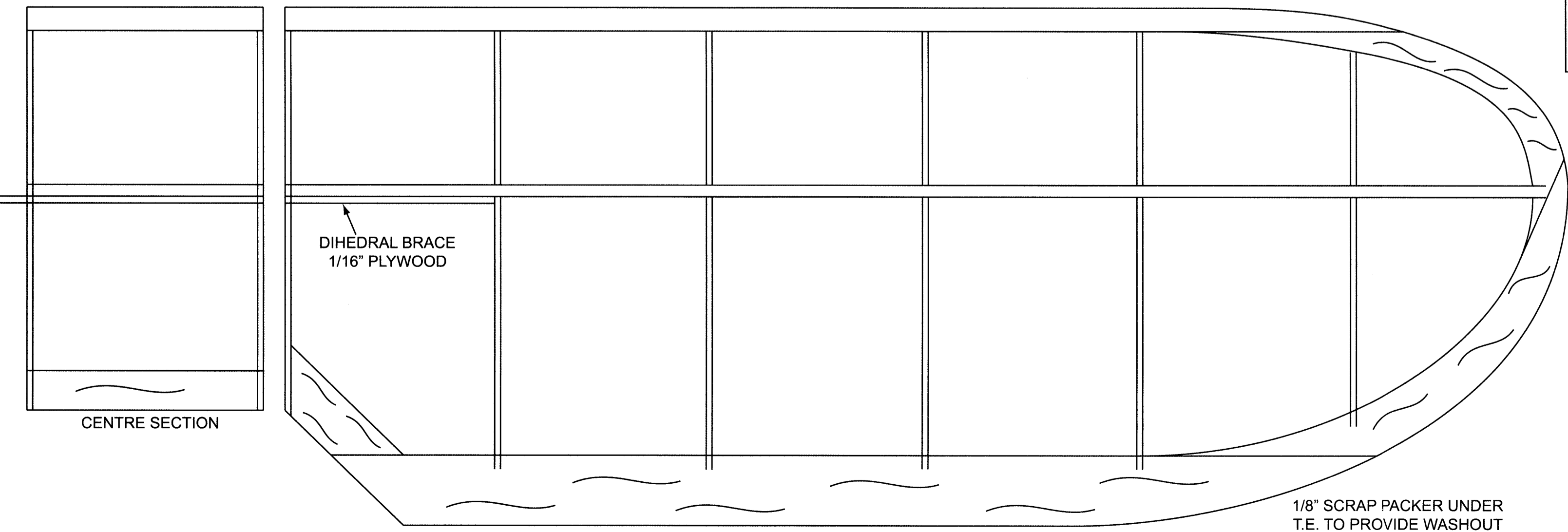
1/16" Balsa SHEET TOP AND BOTTOM OF WING CENTRE SECTION
