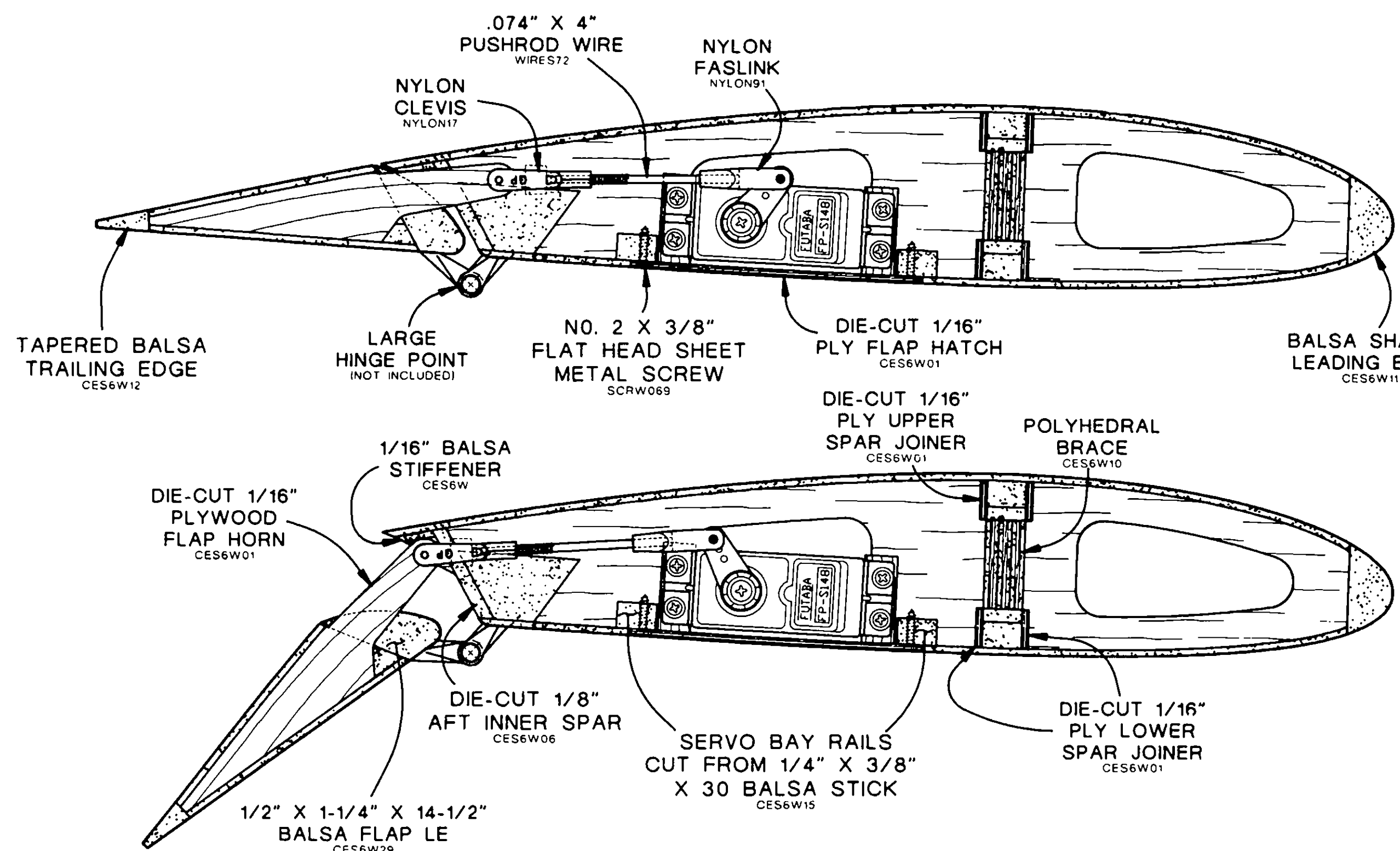
TYPICAL WING CROSS-SECTION SHOWING DETAILS OF FLAPS AND THE FLAP LINKAGE AT RIB W-5
