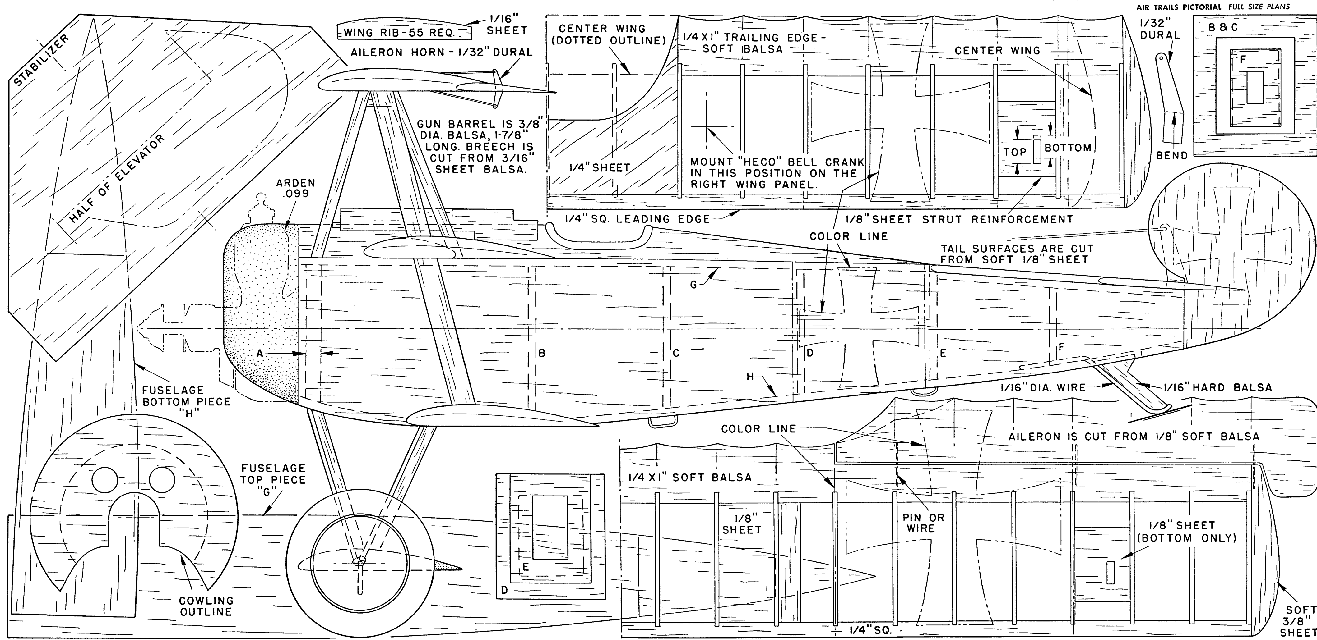
AIR TRAILS PICTORIAL FULL SIZE PLANS
