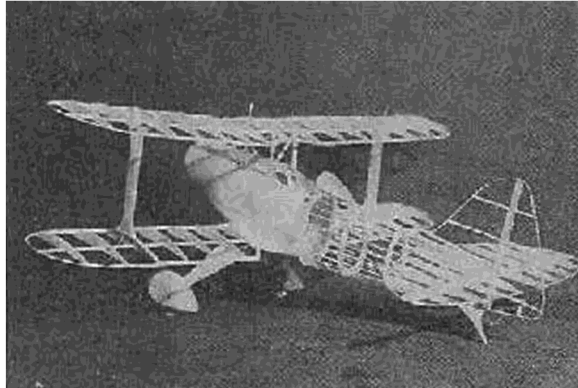
The construction is interesting, having many features seldom found in a flying scale model.
