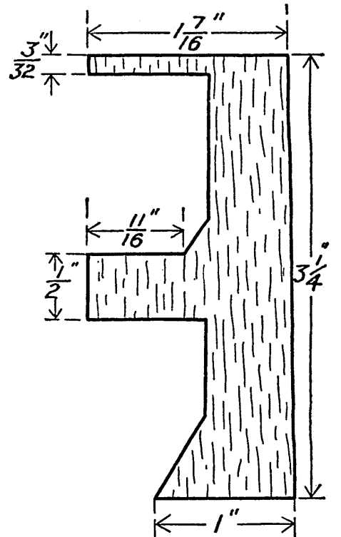
COCKPIT FORMER Make 2
