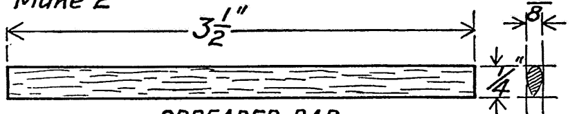
SPREADER BAR 1/4 x 1/8 Balsa, Streamlined
