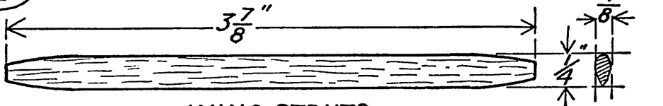
WING STRUTS Make 4
