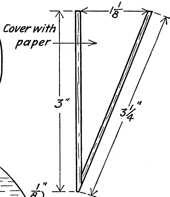
LANDING GEAR Make 2
