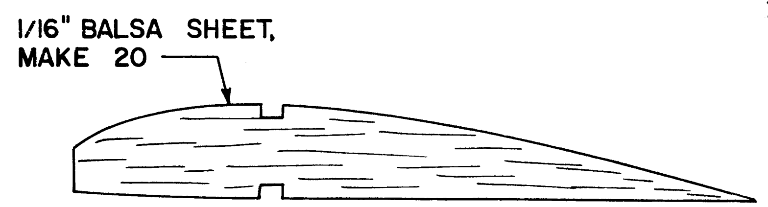
WING RIB PATTERN
