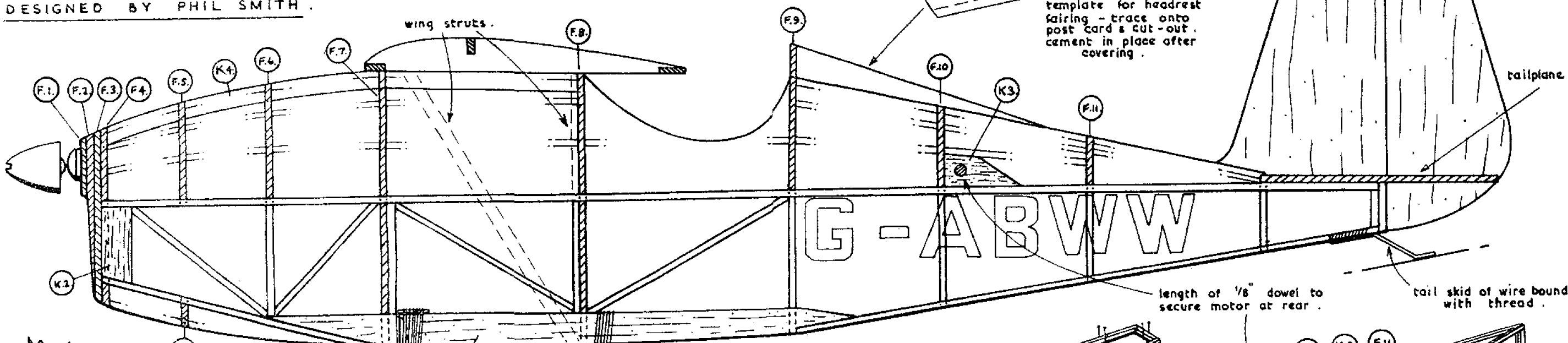
DIAG 1. 1st stage of construction - one side built directly over plan.
