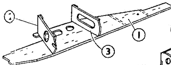
Fig. 1 CEMENT BULKHEADS 2 & 3 IN PLACE FIRST.
