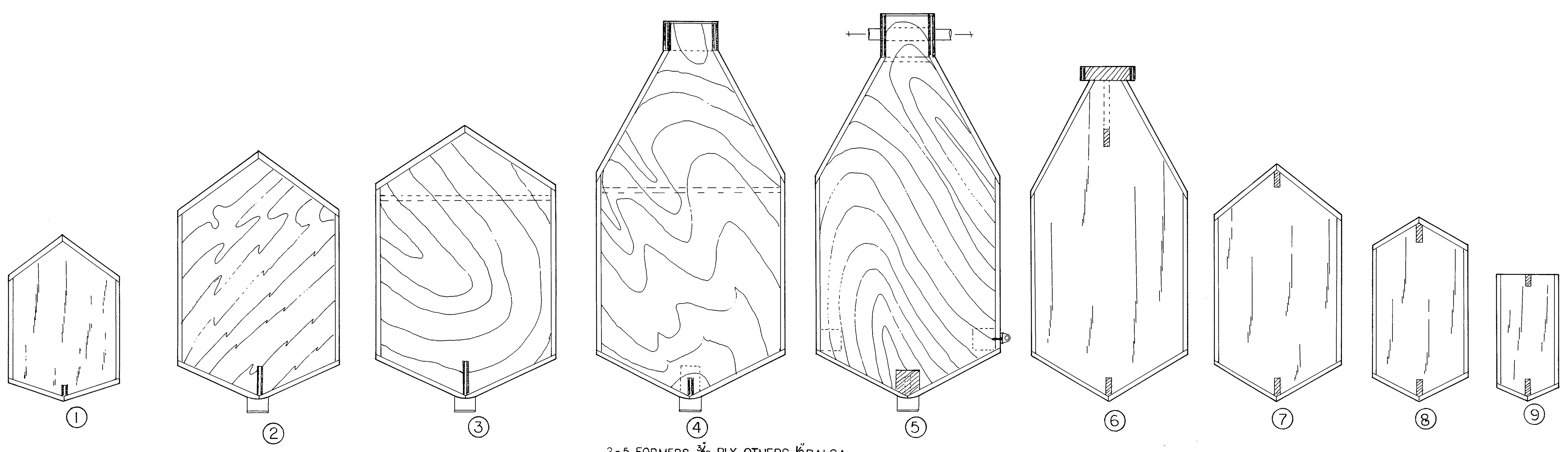
2-5 FORMERS \frac{1}{32} PLY OTHERS \frac{1}{8} Balsa
