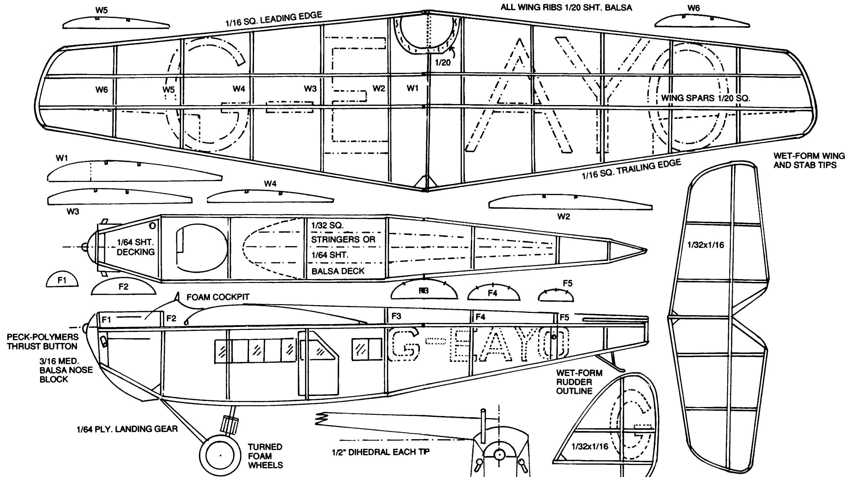
DeHavilland D.H. 29 A 1921 10-Passenger Transport in Peanut Scale Stan Fink 11/2/93
