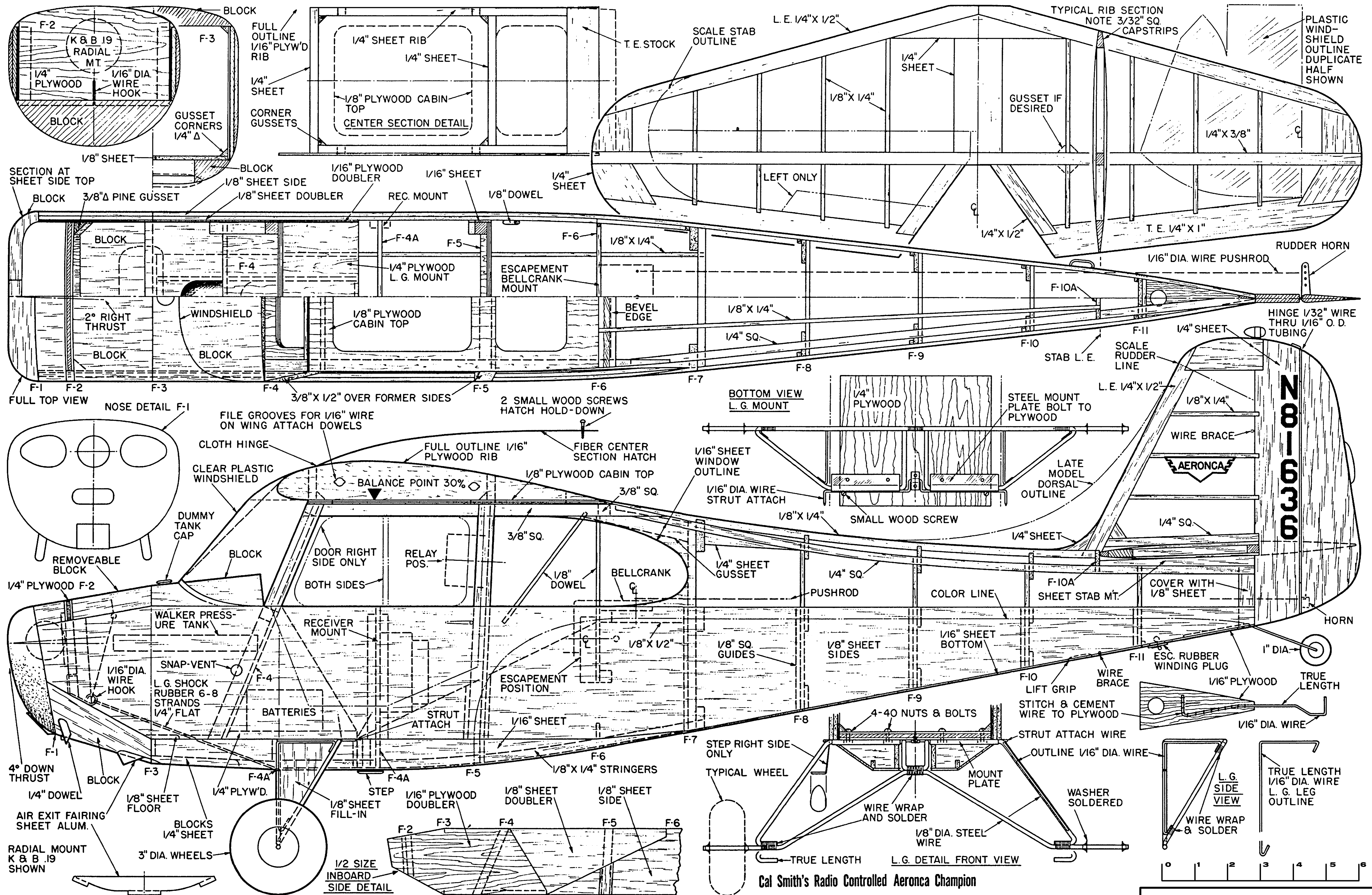
Cal Smith's Radio Controlled Aeronca Champion
