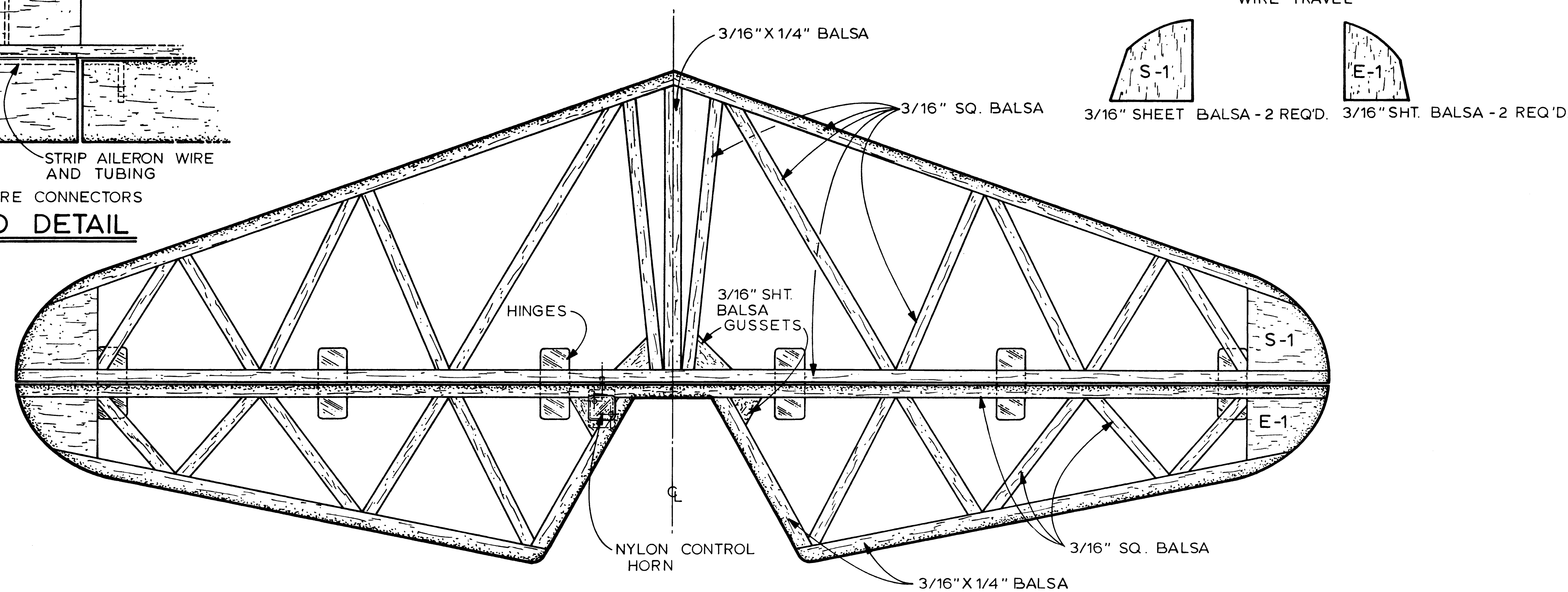
STABILIZER & ELEVATOR PLAN
