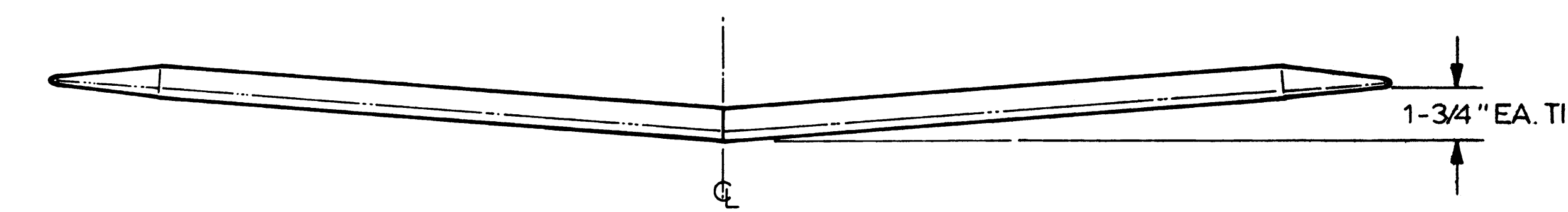
UPPER & LOWER WING DIHEDRAL DETAIL
