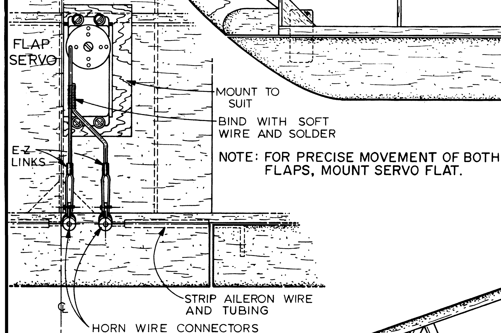
FLAP SERVO DETAIL
