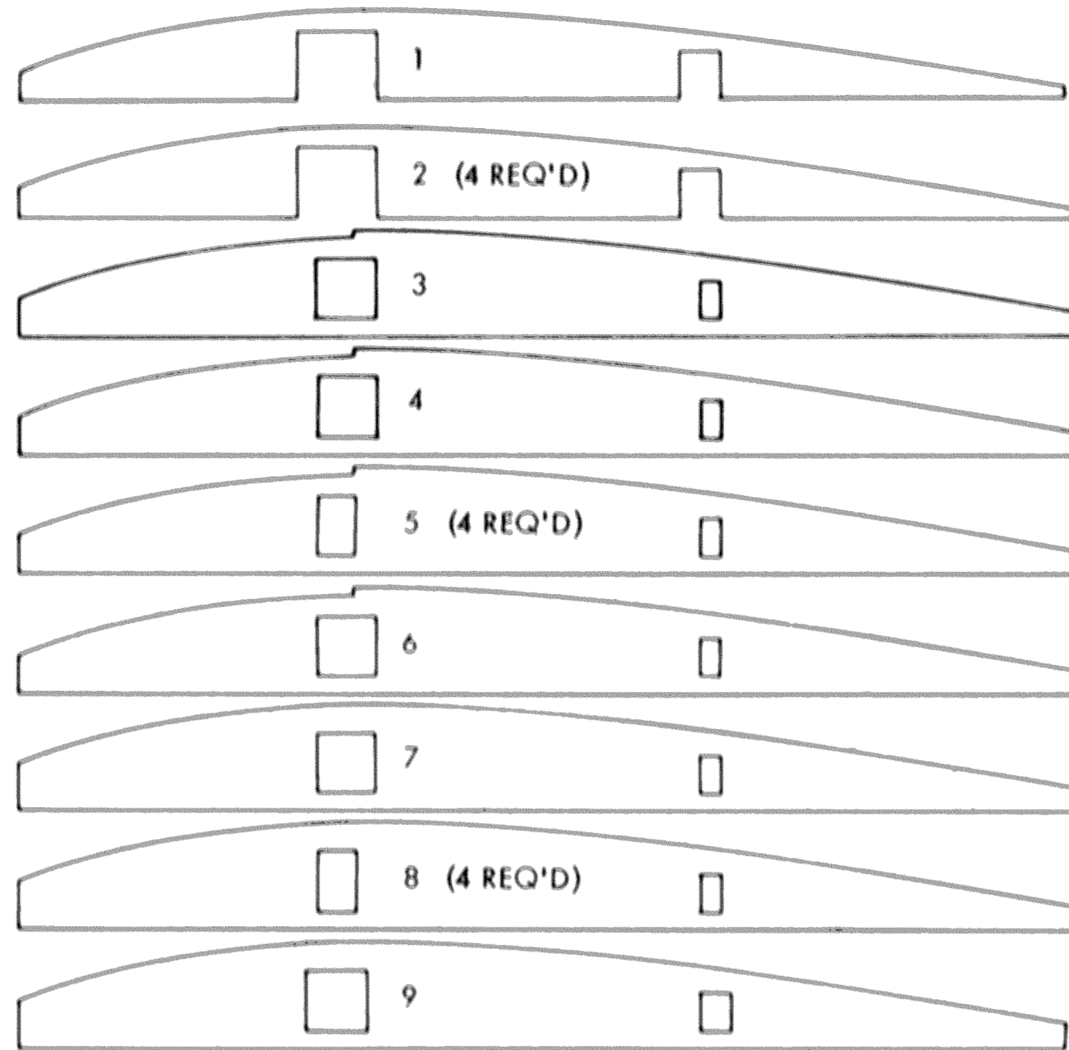
INNER RIBS
