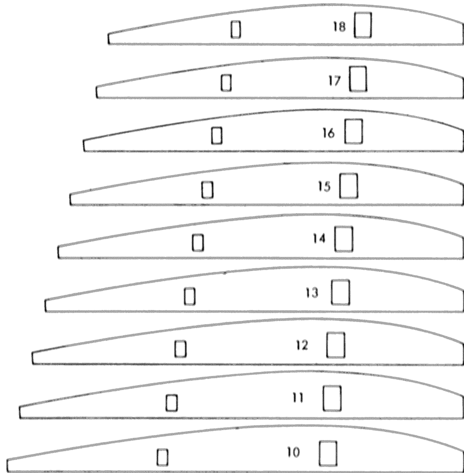
OUTER RIBS
