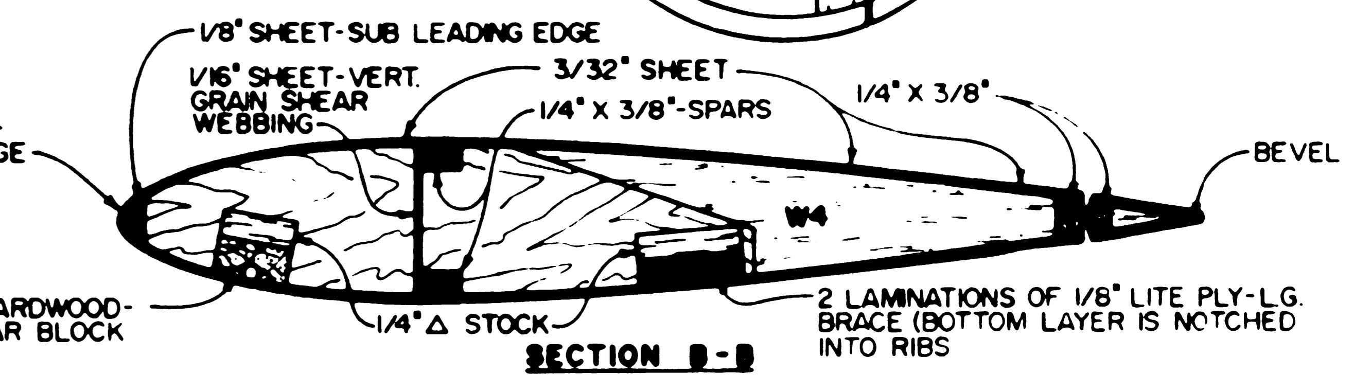
SECTION B-B
