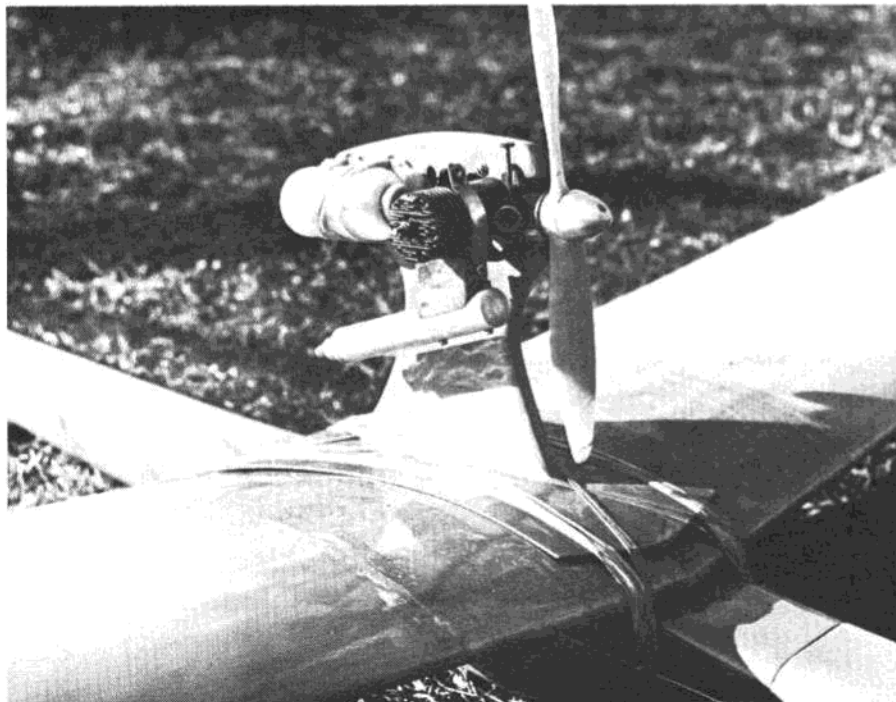
Large engine and small tank work as well as large tank and small engine, but author recommends the fast climb on powerful but light Fox 35 engine. Power pod could be streamlined considerably; it noticeably hinders the glide of King Kong.
