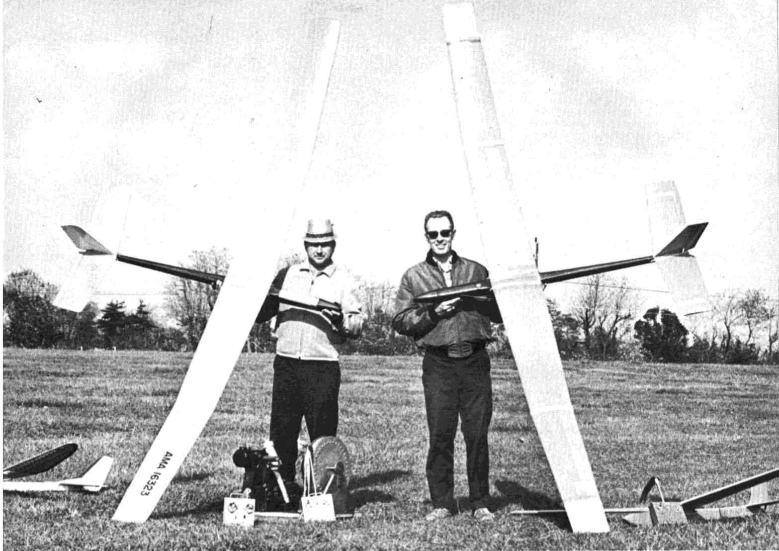
Joe Roslyn and author hold the first two Kongs, still flying after two years! Note use of plastic tape around wing chord at outer dihedral breaks to seal air gap and retain tips. Heavy-duty gas-powered launch winch in foreground.
