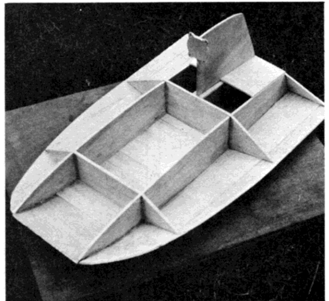
Bottom outside panels attached—the top sheeting started. Side-mounted engine permissible by making modification to mount.
