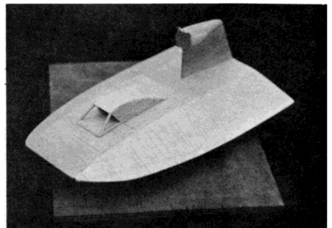
Completed "in the white." Hatch is cut out and the cabin is built. Sanding sealer first step necessary to a sterling finish.
